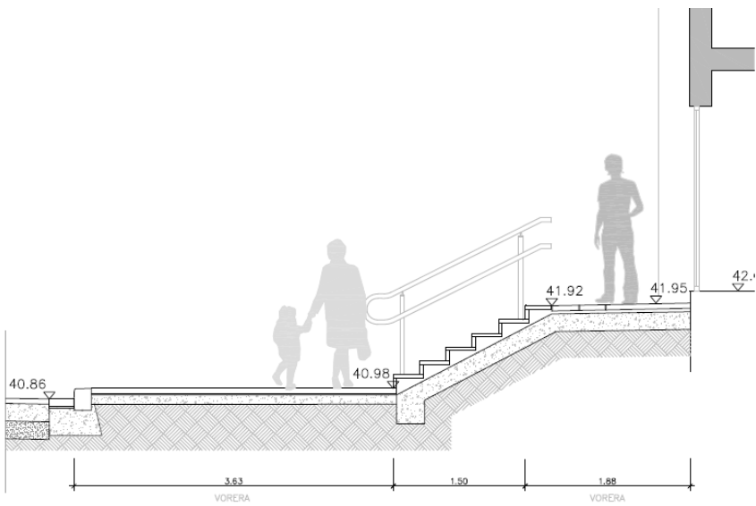
E-E'
